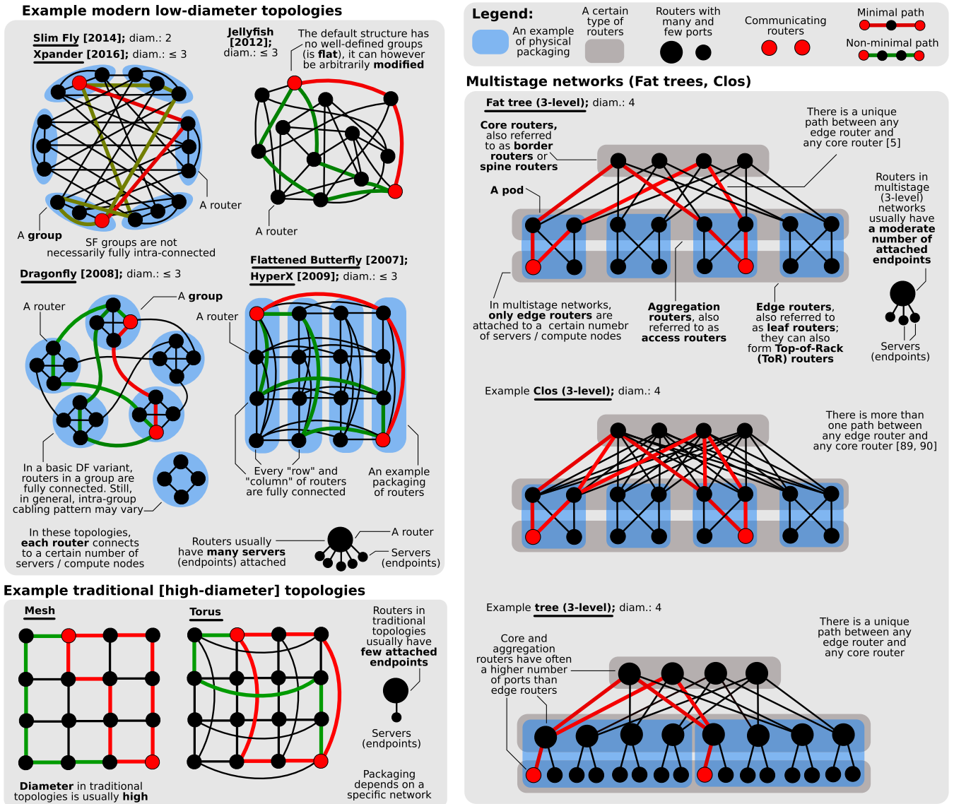
Fig. 3. Illustration of network topologies related to the routing protocols and schemes considered in this work. Red color indicates an example short-path between routers. Green color indicates example alternative non-minimal paths. Blue color illustrates grouping of routers.
